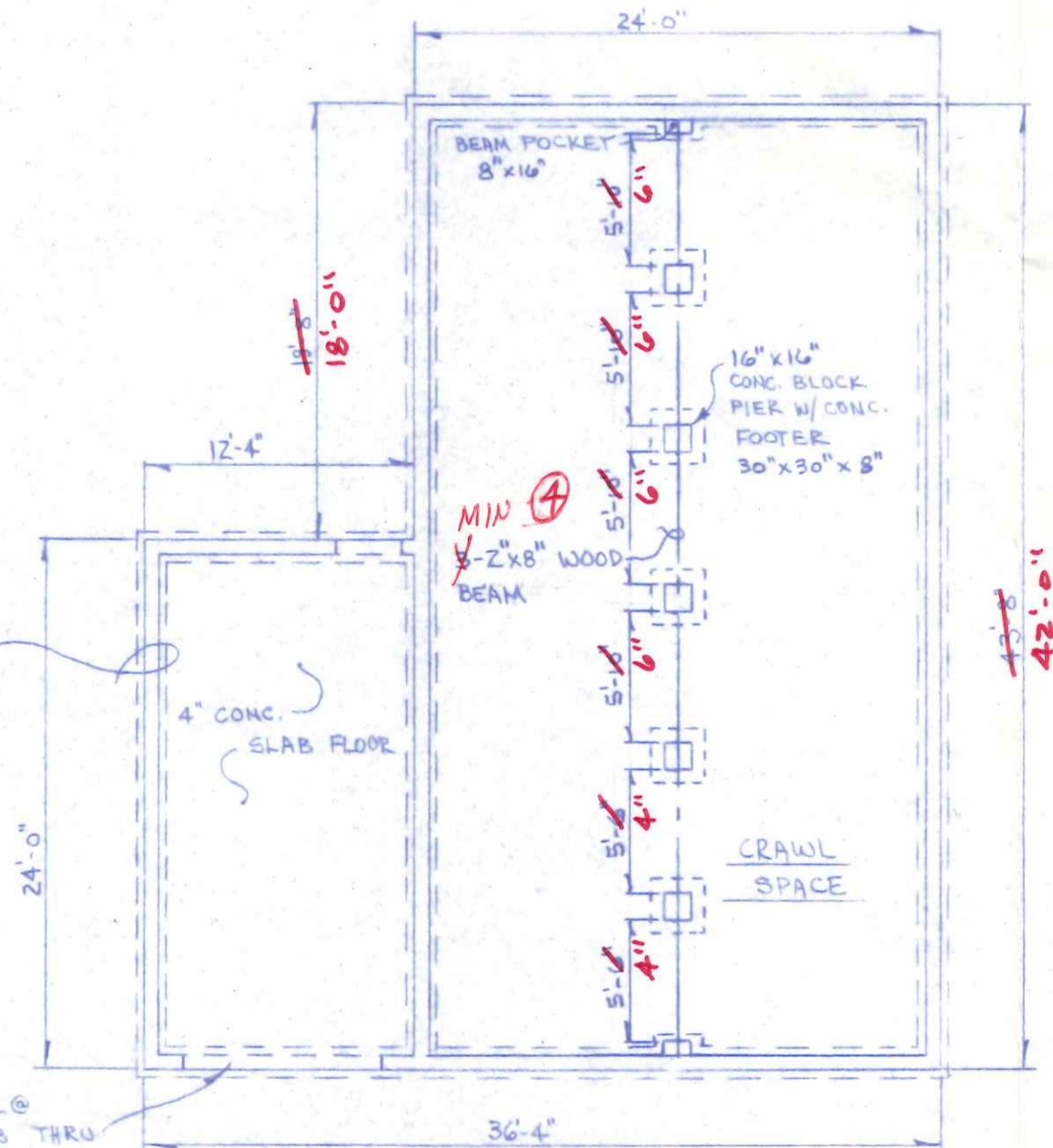
FOUNDATION PLAN 1/8" = 1'-0"
