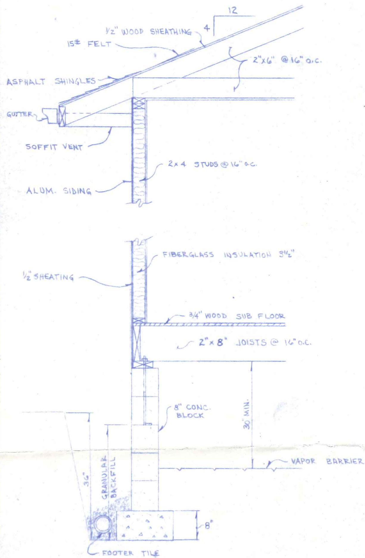
TYPICAL CROSS-SECTION 3/4" = 1'-0"
